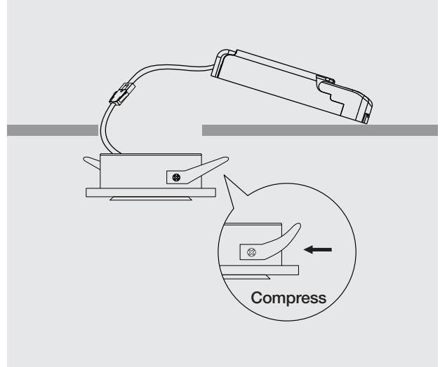
2. Compress spring clips and insert into cutout hole.
